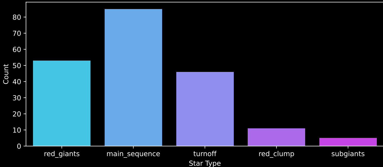
APOGEE DR17 Field: [184+30_MGA] Count plot of Star Type
