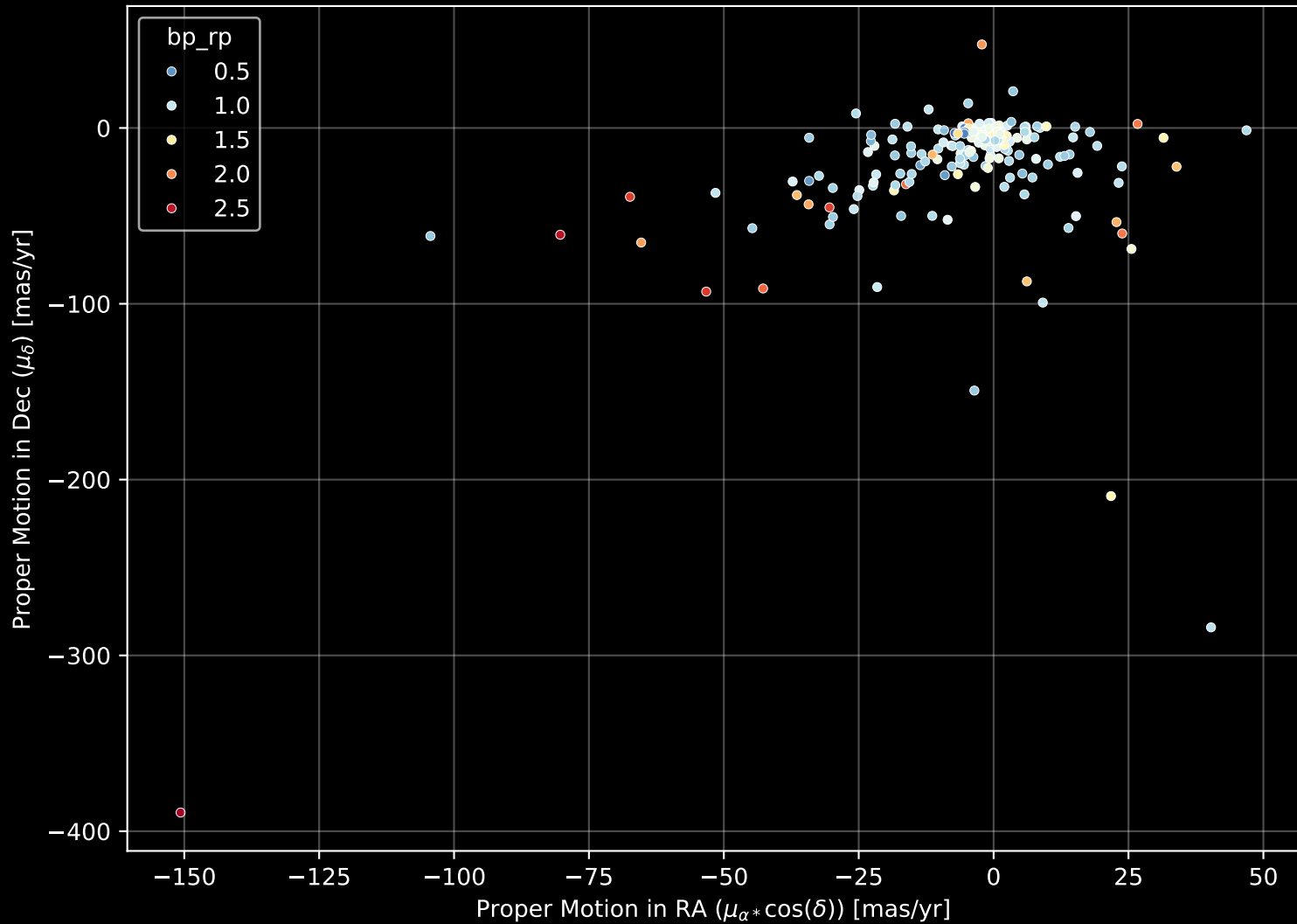
APOGEE DR17 Field: [184+30_MGA] Proper Motion Diagram (n= 200)
