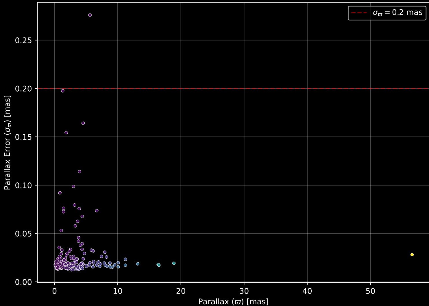
APOGEE DR17 Field: [184+30_MGA] Parallax Quality (n= 200)
