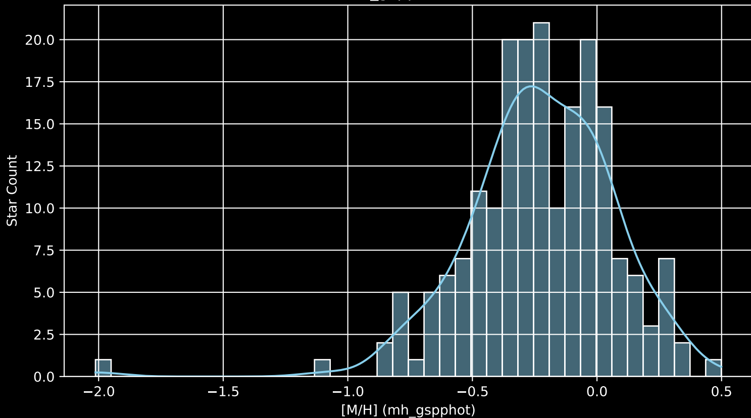
APOGEE DR17 Field: [184+30_MGA [M/H] (mh_gspphot) (n= 198)
