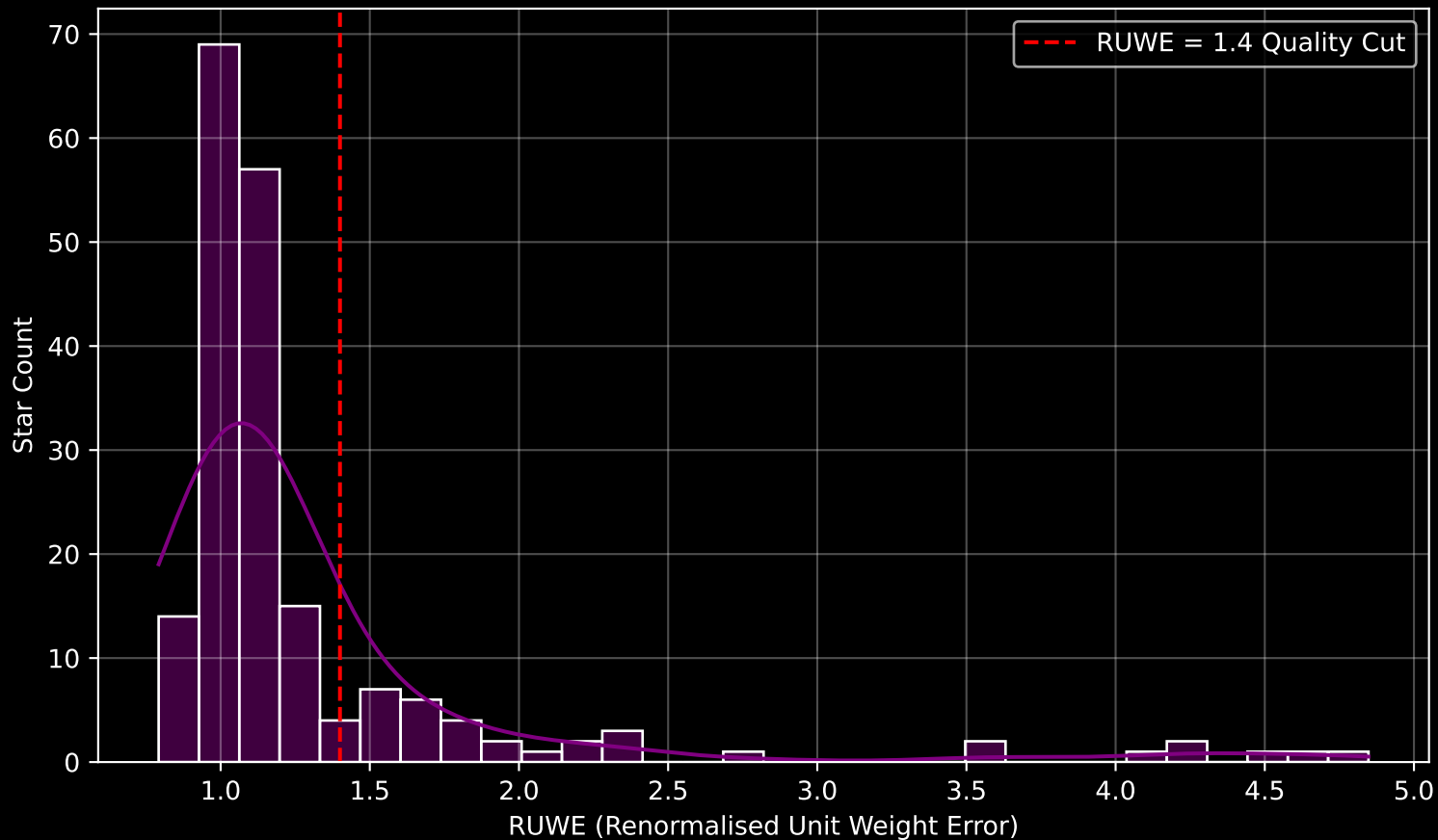
GAPOGEE DR17 Field [184+30_MGA] RUWE Distribution (n= 193)
